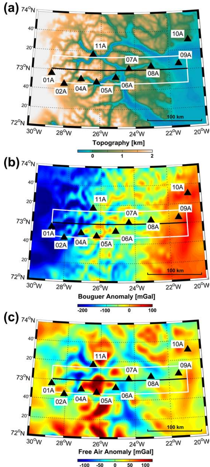
Figure 8. Topography and gravity data in the Central Fjord region. Black triangles – station locations. Stippled black line – position of the section for gravity and seismicological modelling. (a) Topography, (b) Bouguer anomaly and (c) free air anomaly (gravity data from the Arctic data compilation ArcGP (Forsberg & Kenyon 2004; Kenyon et al. 2008)). For the Bouguer gravity a local correlation with topography is due to the lacking terrain correction. In the free air anomaly we observe the fjords and local topographic features standing prominent negative and positive gravity anomalies, respectively, demonstrating isostatic disequilibrium of these small-scale structures.
